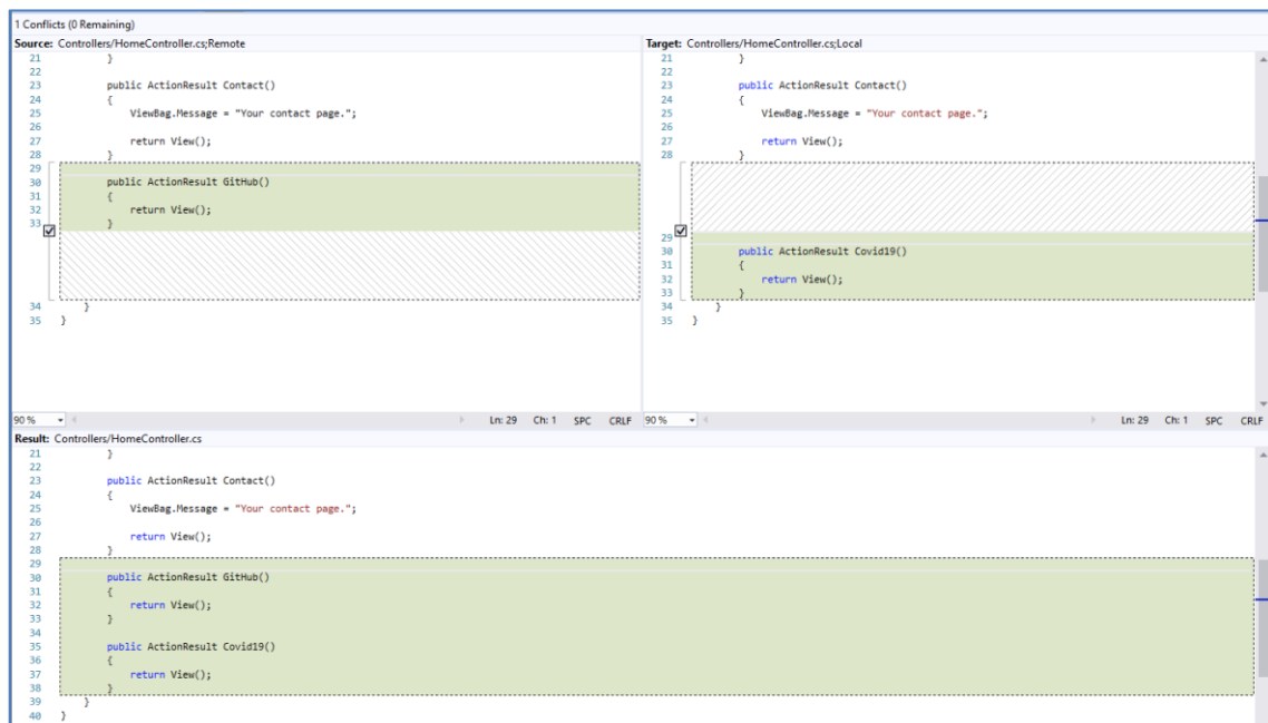
Figure 13. Merging changes in HomeController.cs
