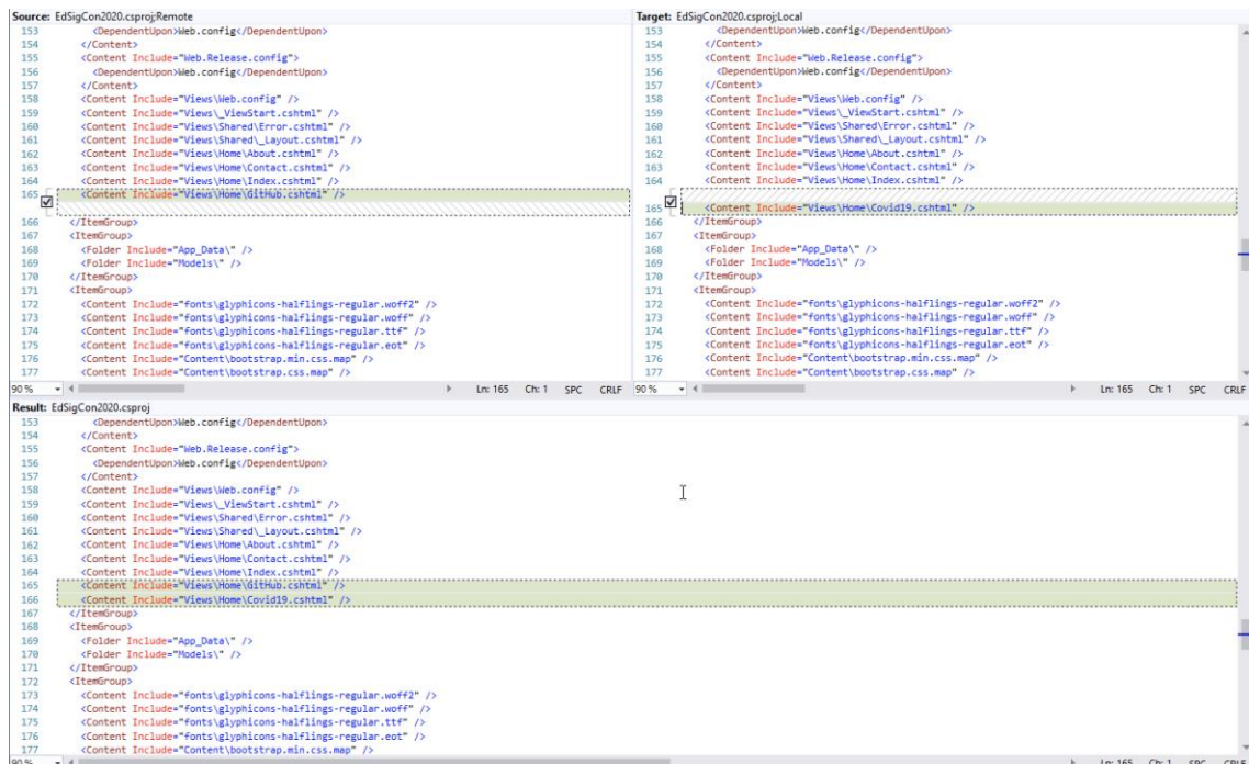
Figure 12. Merging files.
