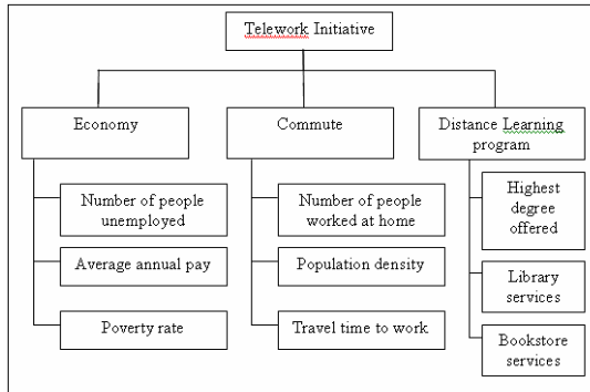
Figure 5.1 Variable Hierarchy
