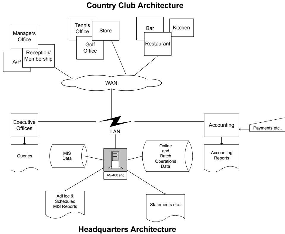
Figure 4: Country Club Billing Application Design
