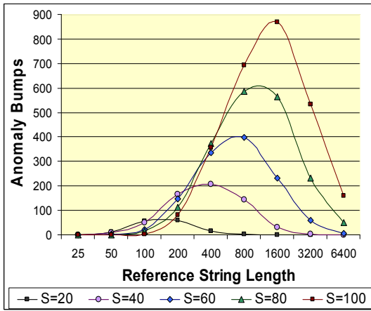
Figure 1. FIFO Anomaly Bumps per 1000 Reference Strings.
