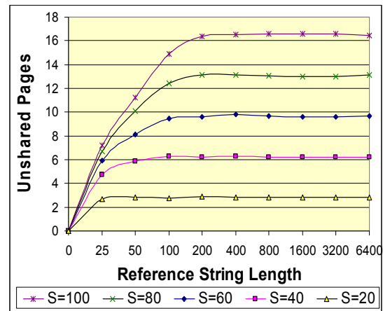
Figure 7. Unshared Pages: Random Page. By process size S and reference string length L. Frames K = 60% of S.
