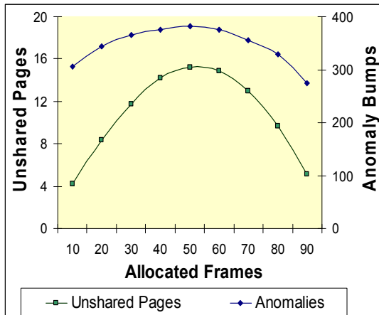
Figure 9. Unshared Pages and Anomalies: Random Page. Process size = 100 and reference string length = 100.
