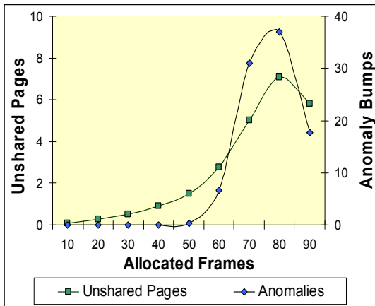
Figure 6. Unshared Pages and Anomalies: FIFO. Process size = 100 and reference string length = 1600.
