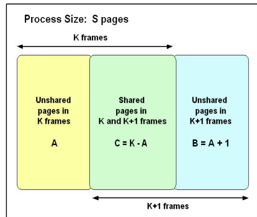
Figure 3. Memory Groups for Page References.
