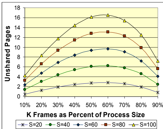
Figure 8. Unshared Pages A and Allocated Frames: Random Page. By process size, using equilibrium A values.
