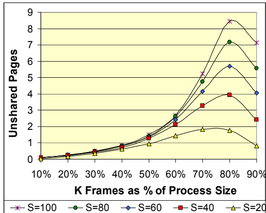
Figure 5. Unshared Pages A and Allocated Frames: FIFO. By process size, using equilibrium A values.
