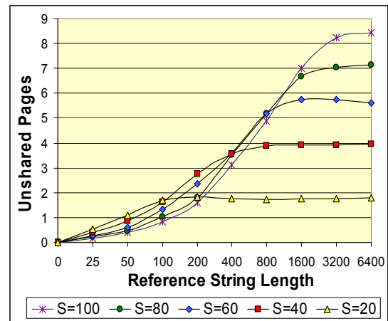
Figure 4. Unshared Pages: FIFO. By process size S and reference string length L . Frames K = 80\% of S .
