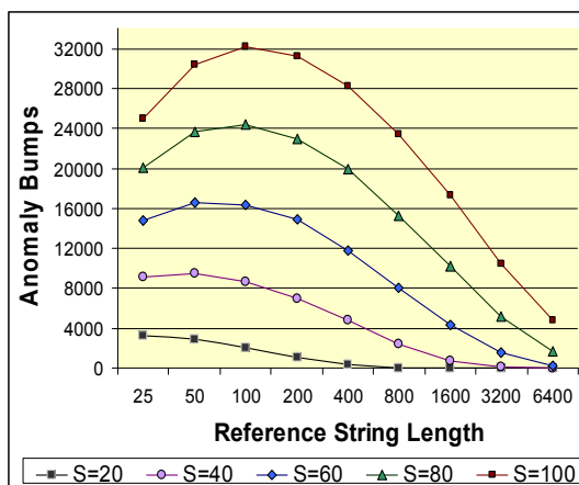
Figure 2. Random Page Anomaly Bumps per 1000 Reference Strings.
